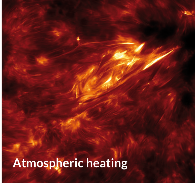
Chromosphere
