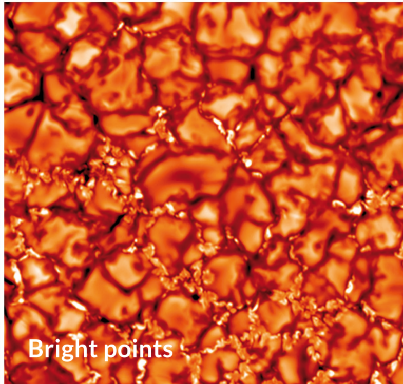
Granulation
