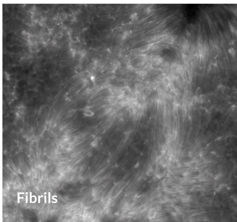
Filaments
