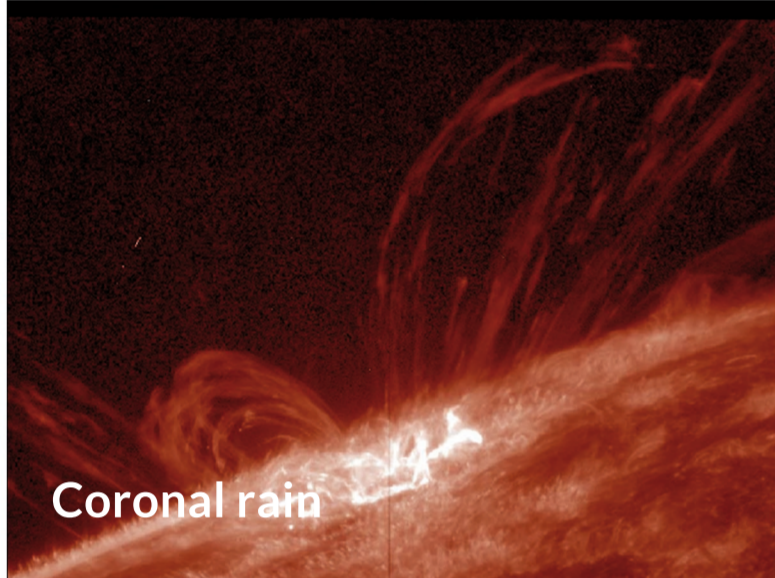
Atmospheric heating
