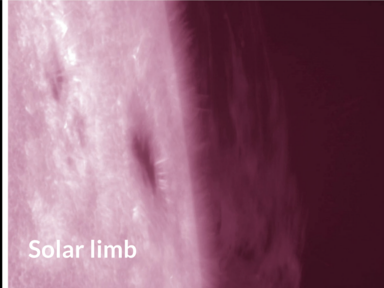
Solar tornadoes
