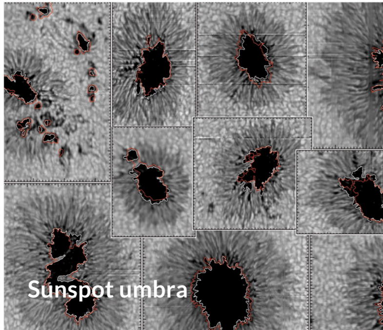
Sunspots
